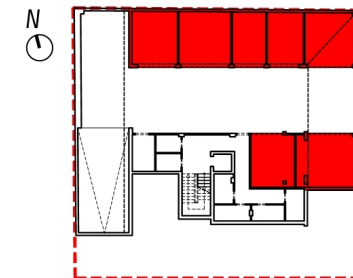
PIANO SEMINTERRATO
